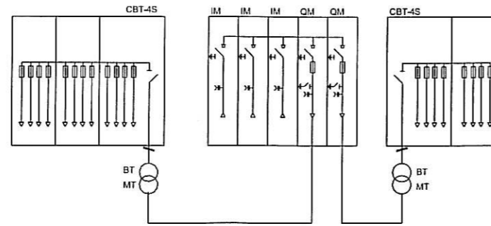
UNIFILAR
